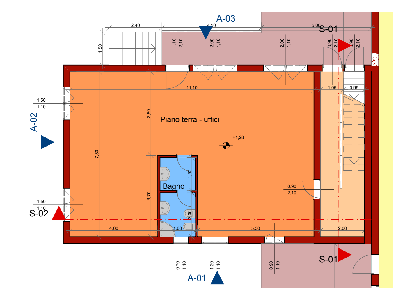
0. PIANO TERRA 1:100
