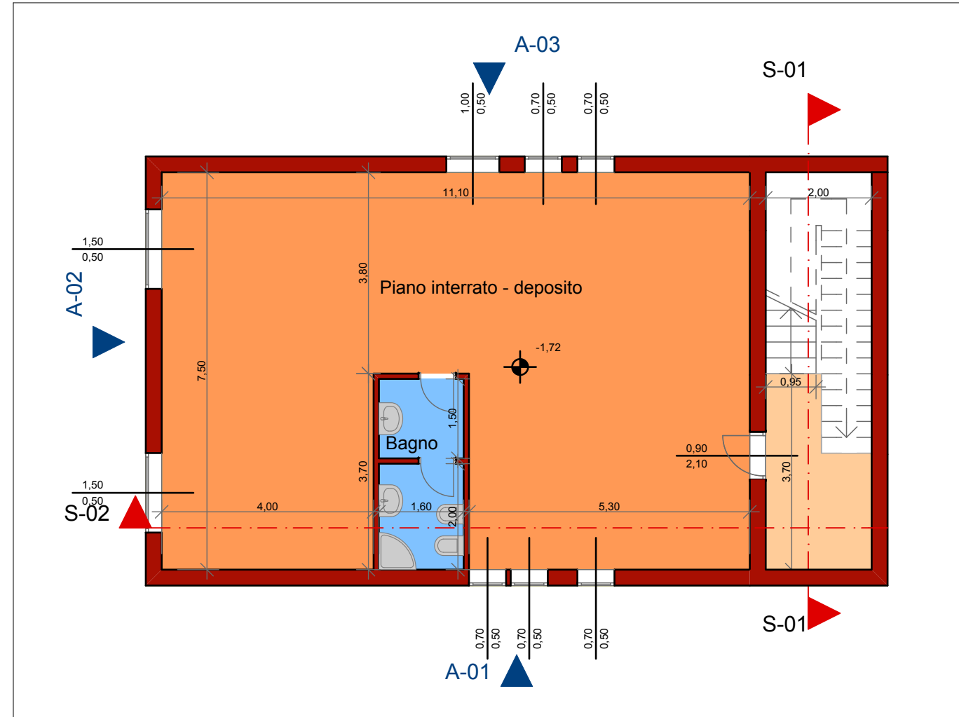
-1. PIANO INTERRATO 1:100
